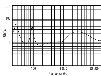
IMPEDANCE
