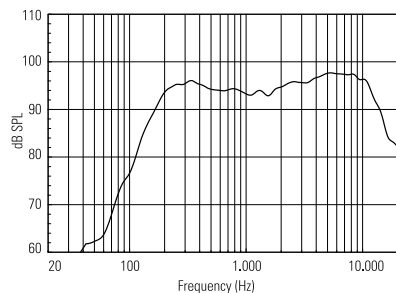
RESPONSE 1W/1m
