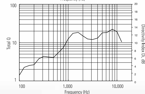
DIRECTIVITY INDEX AND Q
