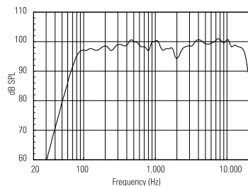
RESPONSE 1W/1m
