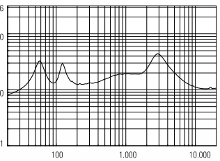
IMPEDANCE
