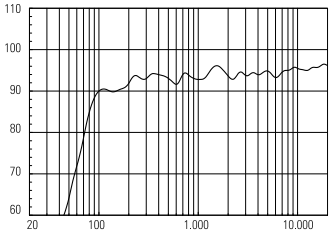
RESPONSE 1W/1m
