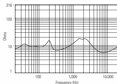
IMPEDANCE
