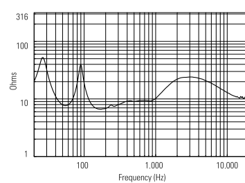
IMPEDANCE
