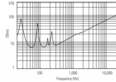
IMPEDANCE
