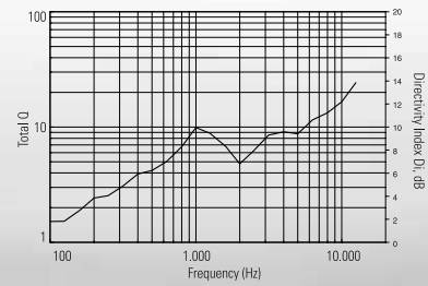
DIRECTIVITY INDEX AND Q
