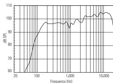
RESPONSE 1W/1m
