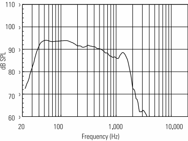
RESPONSE 1W/1m
