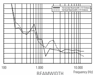
BEAMWIDTH vs. FREQUENCY
