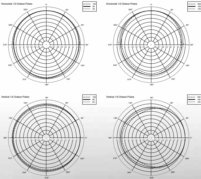
RESPONSE 1W/1m
