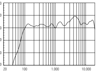
RESPONSE 1W/1m
