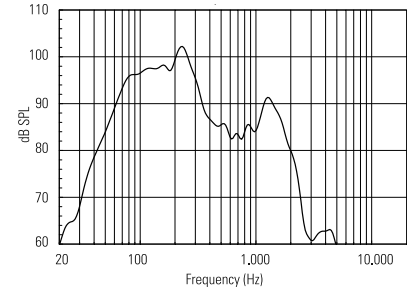
RESPONSE 1W/1m
