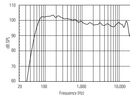
RESPONSE WITH DX4800 PROCESSOR
