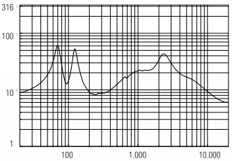
IMPEDANCE
