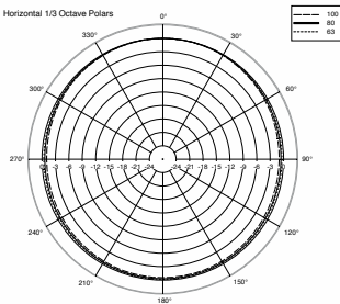
RESPONSE 1W/1m
