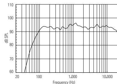
RESPONSE 1W/1m
