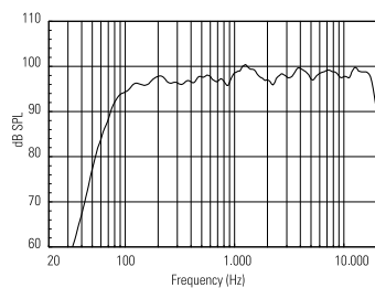
RESPONSE 1W/1m
