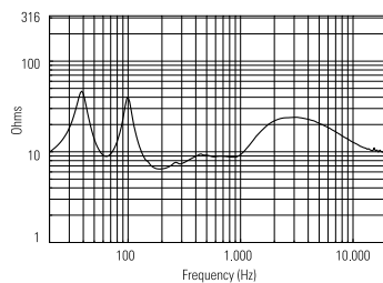
IMPEDANCE
