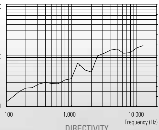
DIRECTIVITY INDEX AND Q
