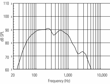
RESPONSE 1W/1m
