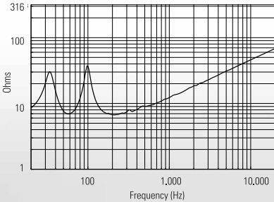
IMPEDANCE
