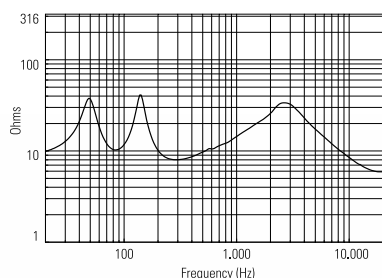
IMPEDANCE
