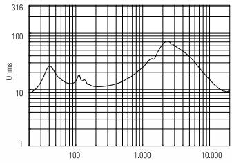
IMPEDANCE
