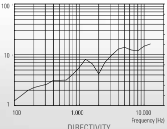
DIRECTIVITY INDEX AND Q
