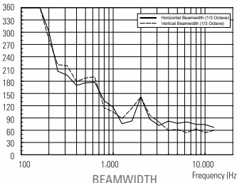
BEAMWIDTH vs. FREQUENCY
