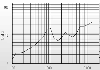
DIRECTIVITY INDEX AND Q
