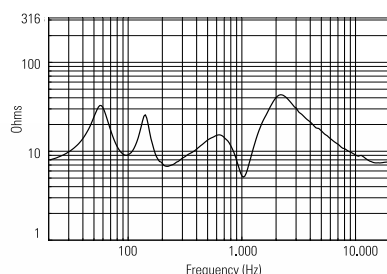
IMPEDANCE
