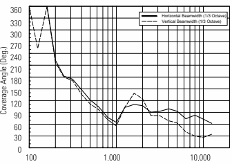
BEAMWIDTH vs. FREQUENCY
