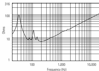
IMPEDANCE
