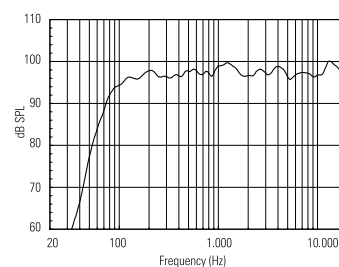
RESPONSE 1W/1m
